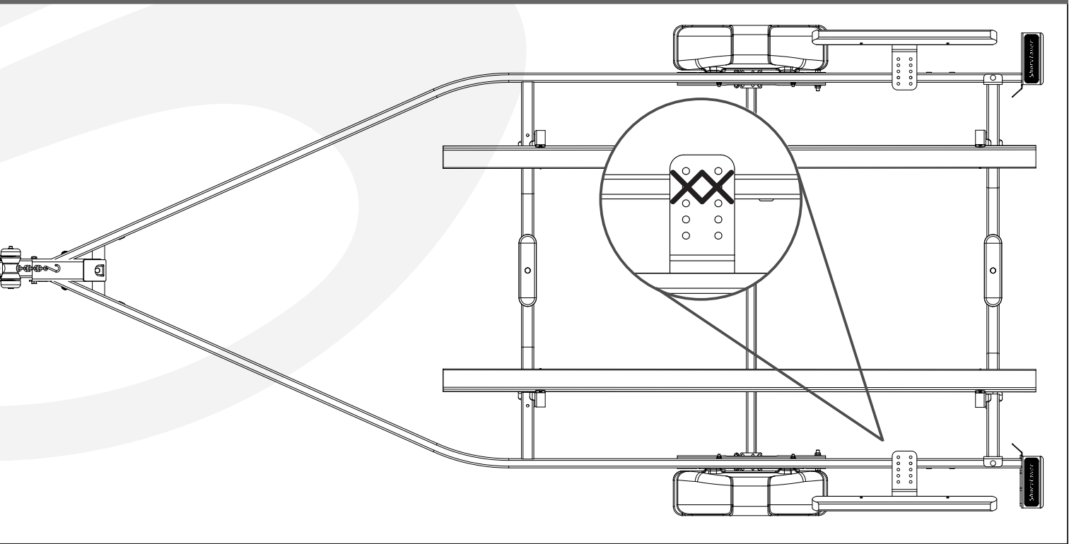
GUIDE-ON BUNK MOUNTING LOCATION
