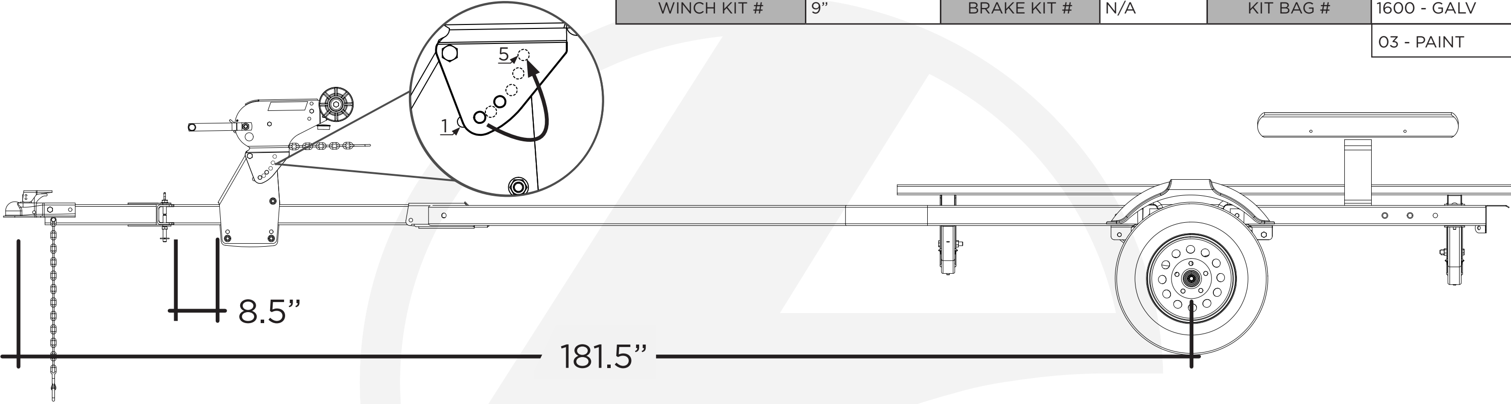
CENTER CROSS SUPPORTS
