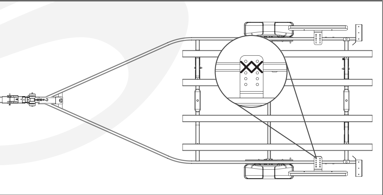
GUIDE-ON BUNK MOUNTING LOCATIONS
